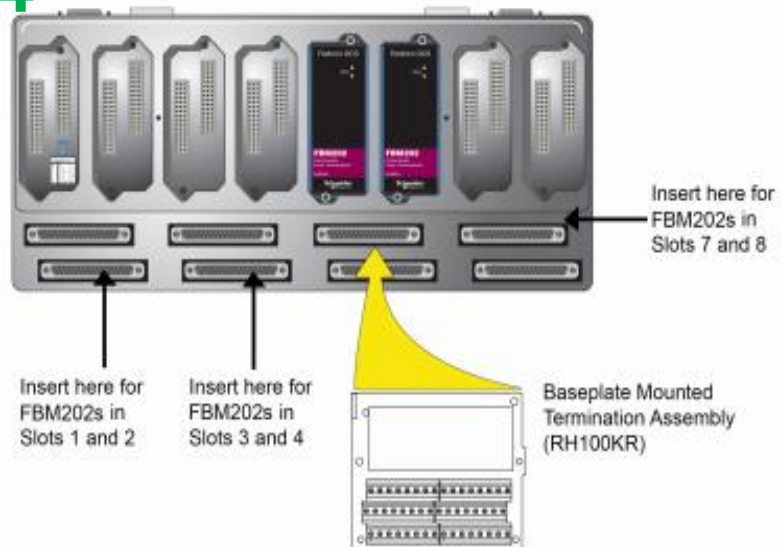
Figure 1 - Baseplate Mounted Termination Assembly
